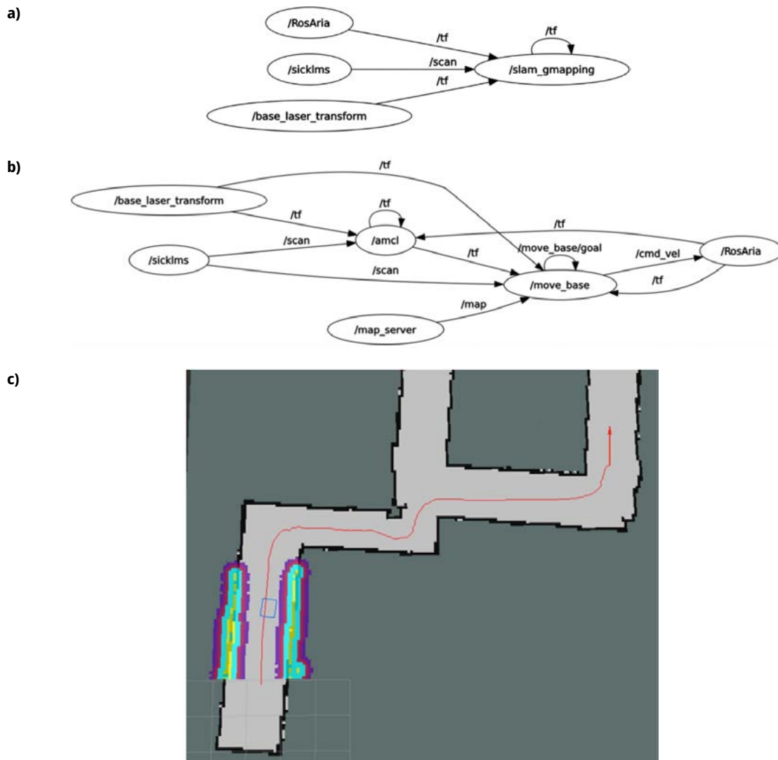
Fig. 2. a) Computational graph of the mapping process. b) Computational graph of the localization and navigation process. c) Cost map for local and global path planning.
